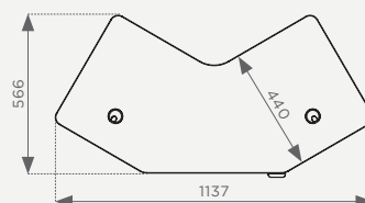
3 ATE-660 Tabletop V-shaped suitable for 2 instruments 1136 x 566 [mm]
